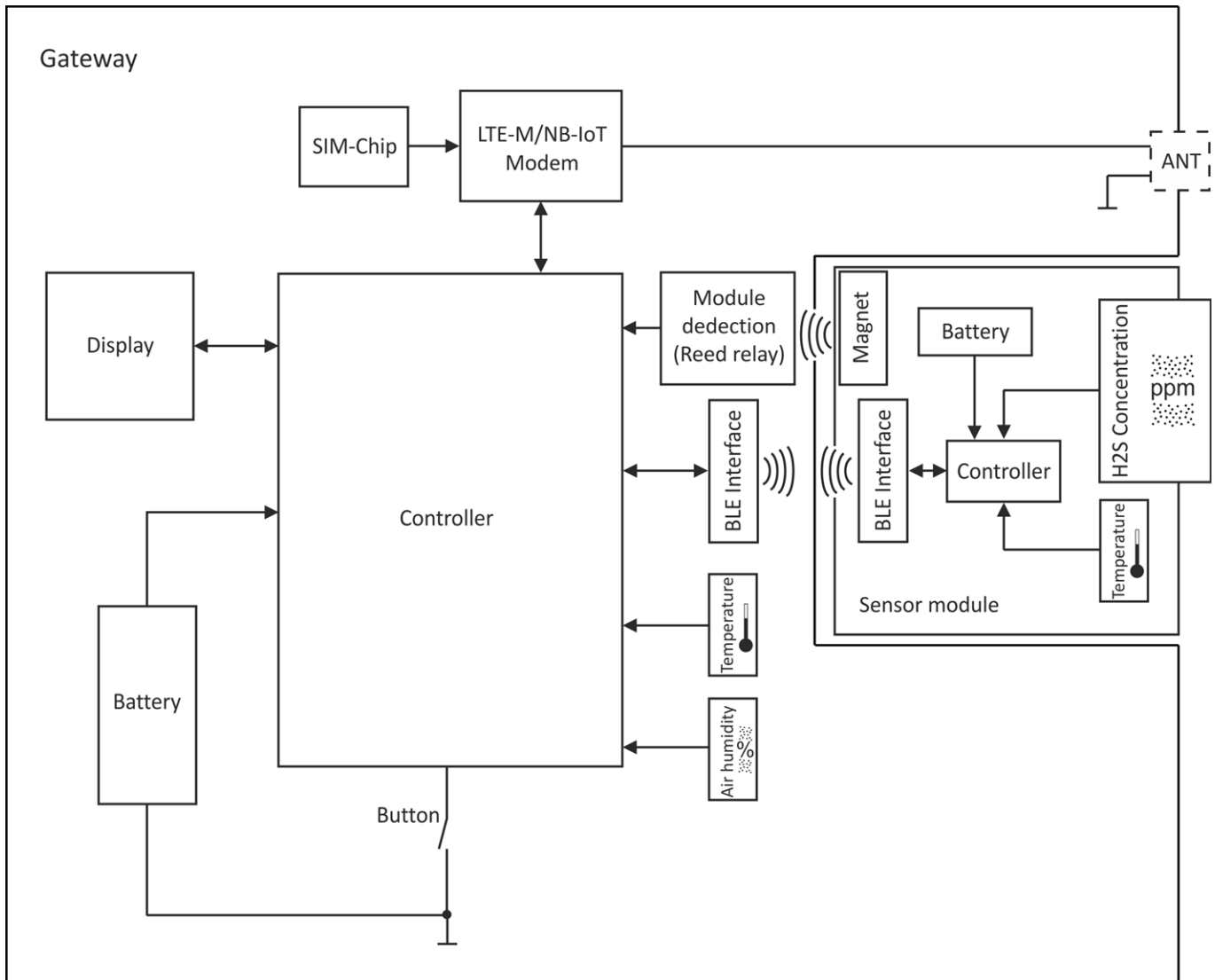
Block diagram of the myDatasensH2S1000 LTE-M
