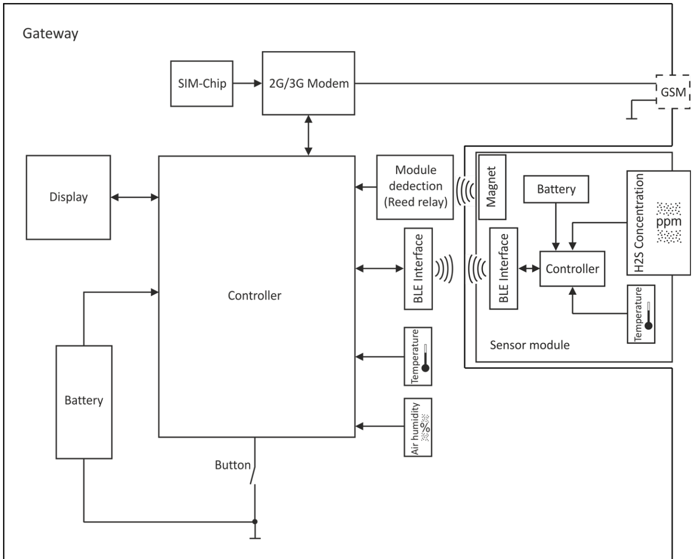
Block diagram of the myDatasensH2S1000 BLE & 3G
