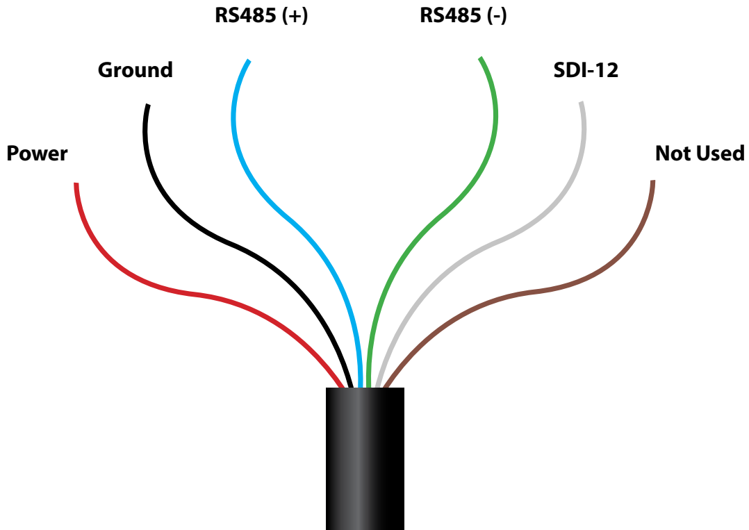
Stripped and Tinned Cable Wire Legend
